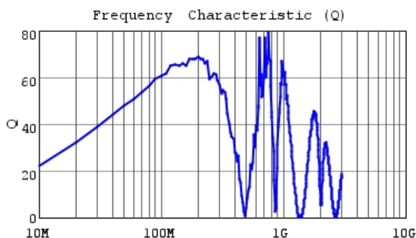
LQW2UASR68F00 Q
