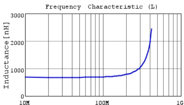
LQW2UASR68F00 L
