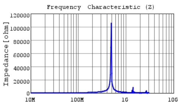
LQW2UASR68F00 |Z|
