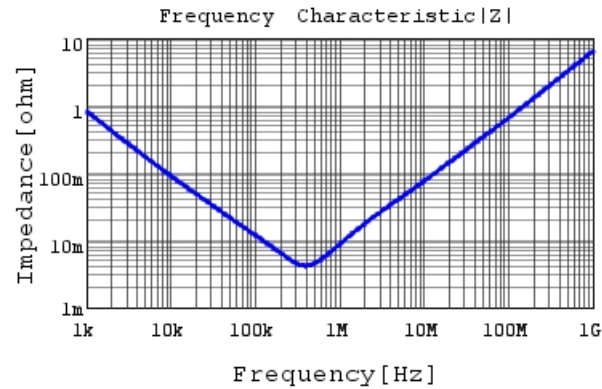
ECASD40J227M010KA0 |Z| DCOV, 25degC
