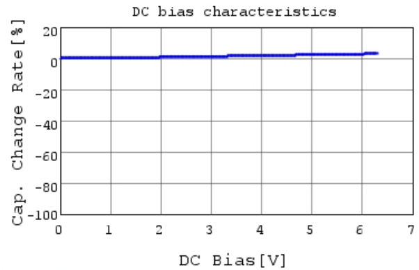
ECASD40J227M010KA0 C-DC bias capchange, 25.0
