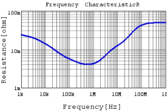
ECASD40J227M010KA0 R DCOV, 25degC
