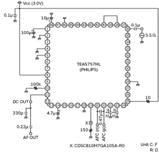
Measurement Circuit
