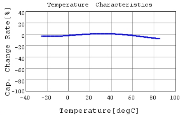
DE1B3KX331KA4BP01F C-Temp. capchange, DCOV,
