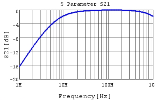
DE1B3KX331KA4BP01F S21 DCOV, 20degC
