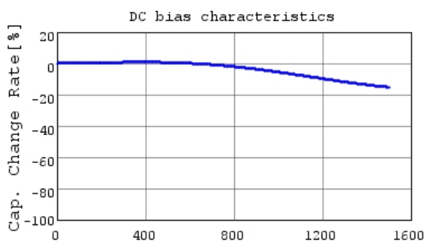
DE1B3RA221KA4BQ01F C-DC bias capchange, 20.0
