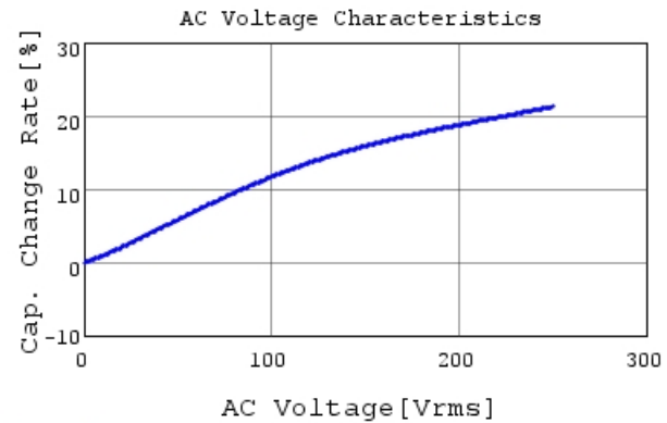
DE1B3RA221KN4AN01F C-AC Voltage capchange, 1
