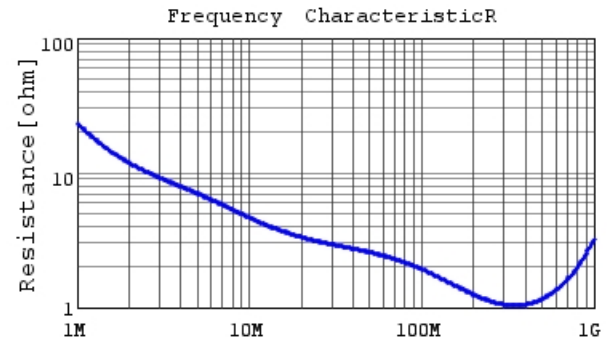
DE1B3RA221KN4AP01F R DCOV, 20degC
