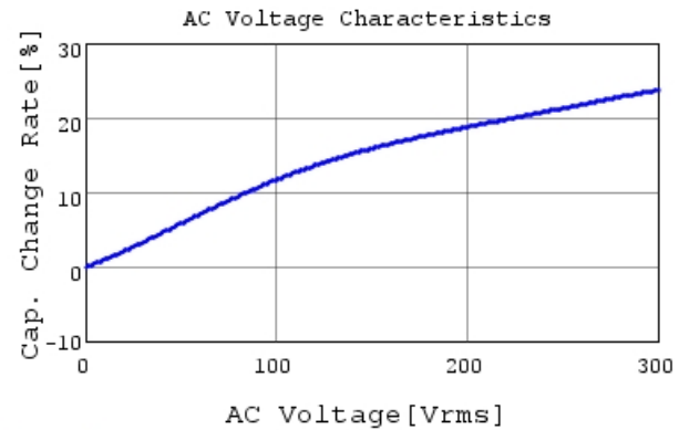
DE1B3RA221KN4AP01F C-AC Voltage capchange, 1
