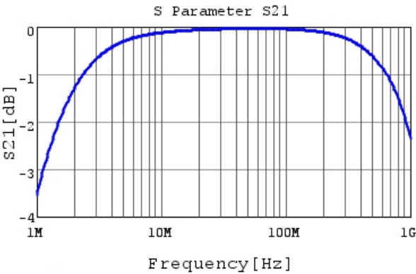
DE1E3RA152MN4AN01F S21 DCOV, 20degC
