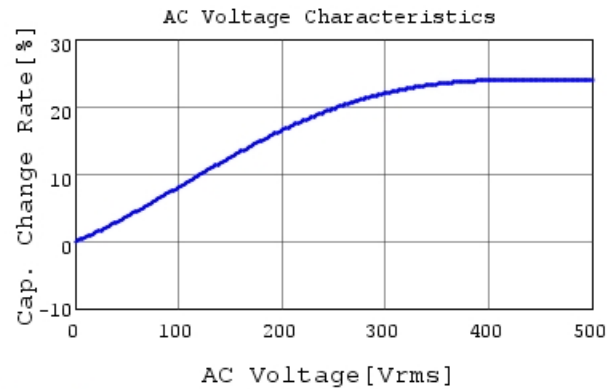
DE1E3RB472MN4AR01F C-AC Voltage capchange, 1
