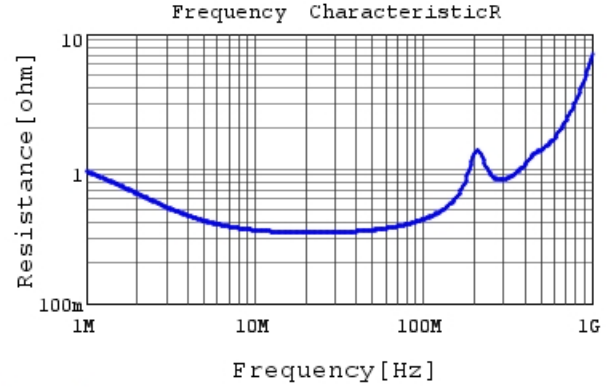
DE1E3RB472MN4AR01F R DCOV, 20degC
