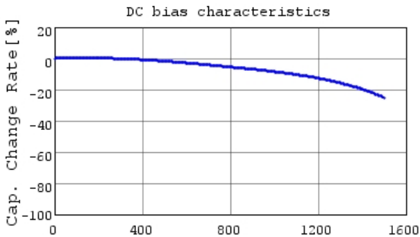
DE2B3SA101KA3BX02F C-DC bias capchange, 20.0
