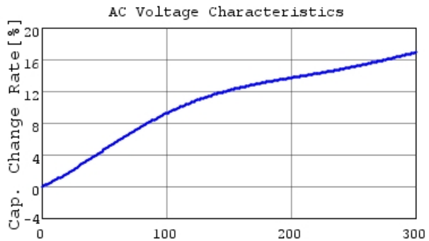
DE2B3SA101KA3BX02F C-AC Voltage capchange, 1
