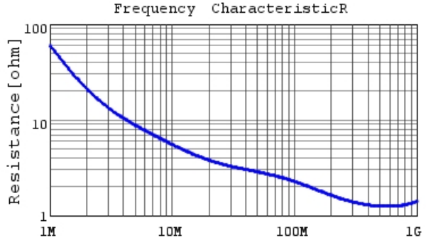
DE2B3SA101KA3BX02F R DCOV, 20degC
