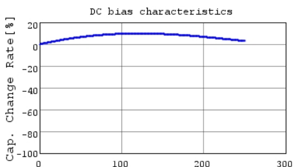
DE2E3KY472MN3AM02F C-DC bias capchange, 20.0
