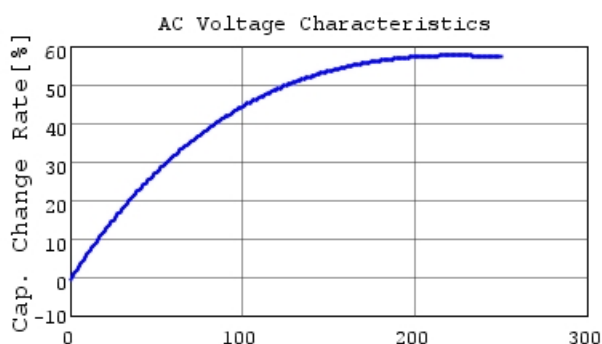
DE2E3KY472MN3AM02F C-AC Voltage capchange, 1
