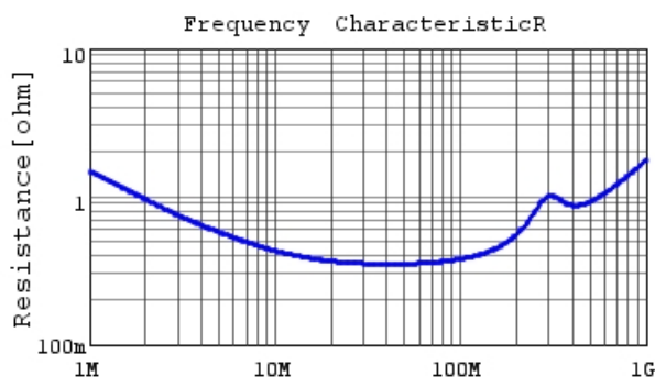
DE2E3KY472MN3AM02F R DCOV, 20degC
