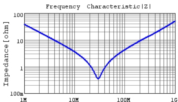
DE2E3KY472MN3AM02F |Z| DCOV, 20degC
