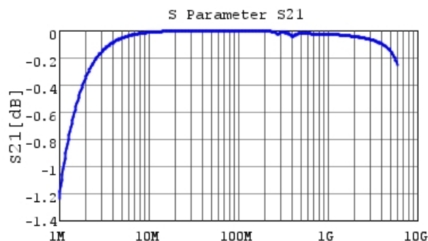
GRM1885C1H272JA01 S21 DCOV, 25degC
