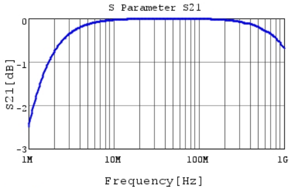
RHE5G1H182J0M1H03A S21 DCOV, 25degC
