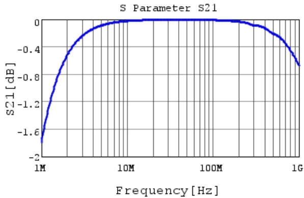
RHE5G1H222J0M1H03A S21 DCOV, 25degC
