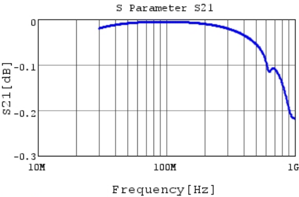
RHE5G1H821J0A2H03B S21 DCOV, 25degC
