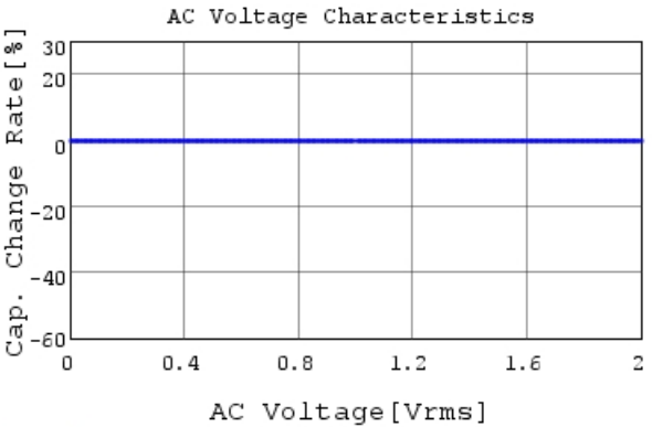
RHE5G2A102J0DBH03A C-AC Voltage capchange, I
