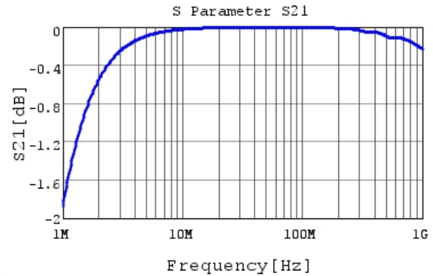
RHE5G2A222J1DBH03A S21 DCOV, 25degC
