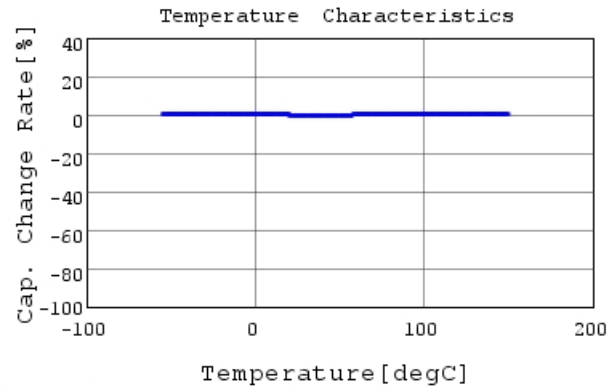
RHE5G2A222J1DBH03A C-Temp. capchange, DCOV,
