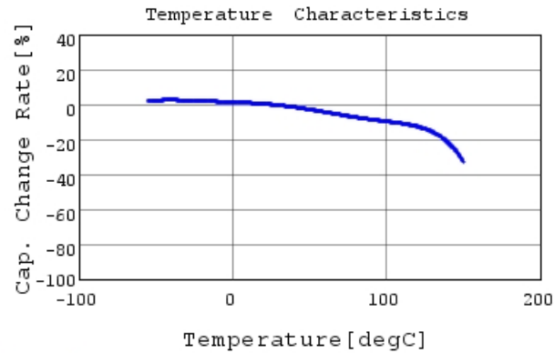
RHEL81E106K3K1H03B C-Temp. capchange, DCOV,
