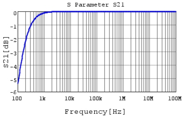
RHEL81E106K3K1H03B S21 DCOV, 25degC
