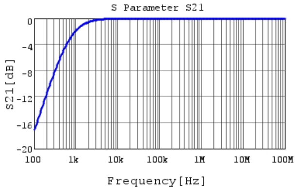
RHEL81E225K2DBH03A S21 DCOV, 25degC
