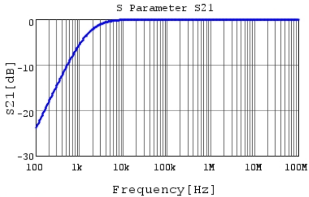
RHEL81H105K2K1H03B S21 DCOV, 25degC
