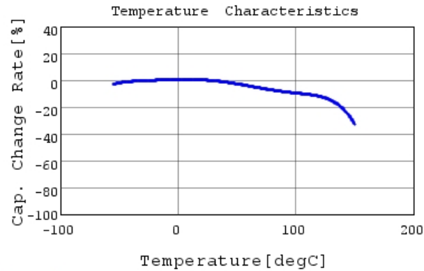
RHEL81H105K2K1H03B C-Temp. capchange, DCOV,
