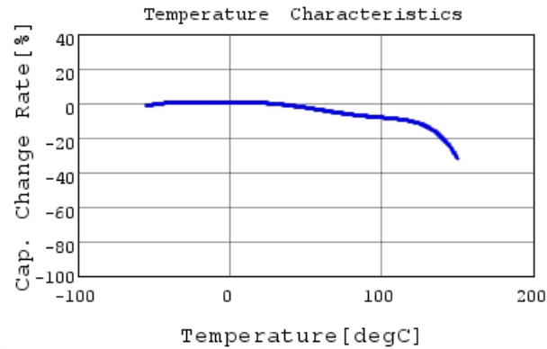
RHEL81H474K2M1H03A C-Temp. capchange, DCOV,
