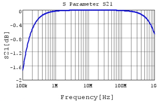
RHEL82A223K0K1H03B S21 DCOV, 25degC
