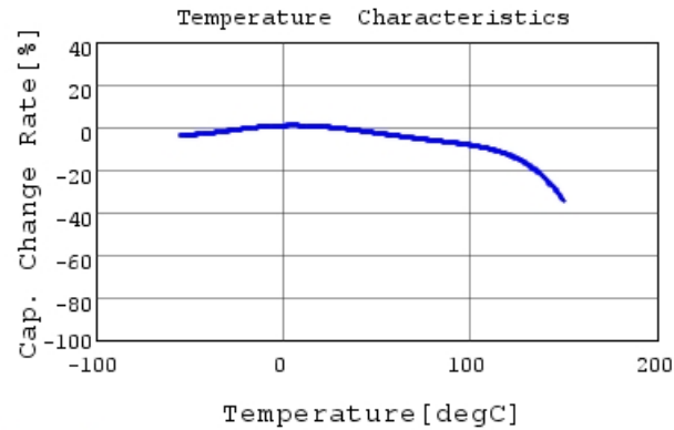
RHEL82A223K0K1H03B C-Temp. capchange, DCOV,
