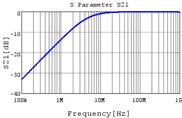
RHEL82A331K0A2H03B S21 DCOV, 25degC
