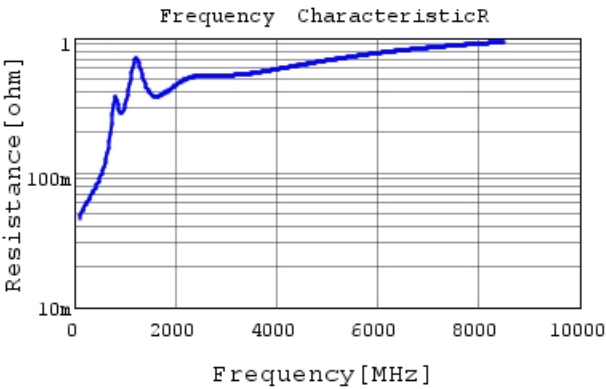
GCM1555C1H561FA16 R DCOV,25degC
