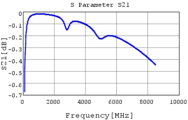
GCM1555G1H390JA16 S21 DC0V, 25degC
