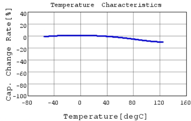
GCM155R71E473KA55 C-Temp. capchange, DC0.0V,
