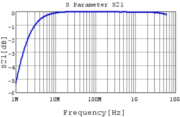
GCM1885C2A102JA16 S21 DCOV, 25degC
