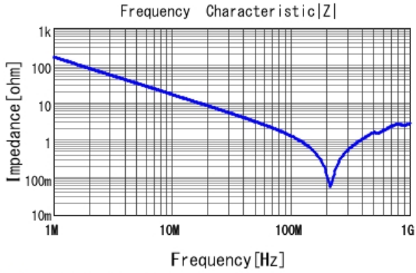
GCM21A5C2E102JX01 |Z| DCOV, 25degC
