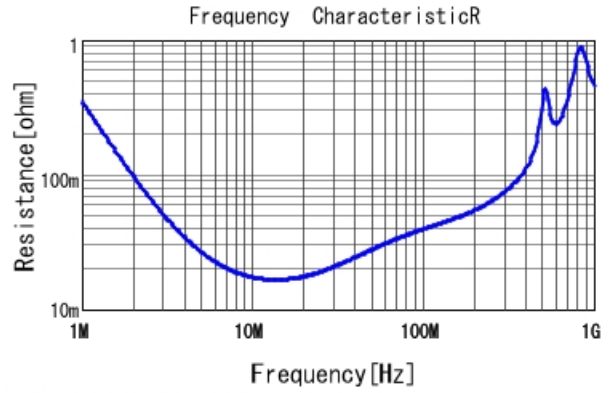
GCM21A5C2E102JX01 R DCOV, 25degC
