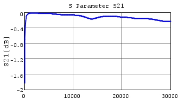
GRM0115C1C220JE01 S21 DCOV, 25degC
