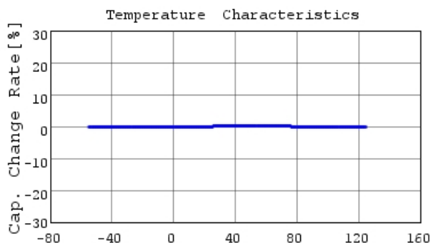
GRM0115C1C220JE01 C-Temp. capchange, DCOV, 1
