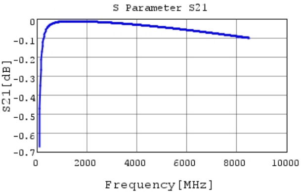
GRM0115C1C390JE01 S21 DCOV, 25degC
