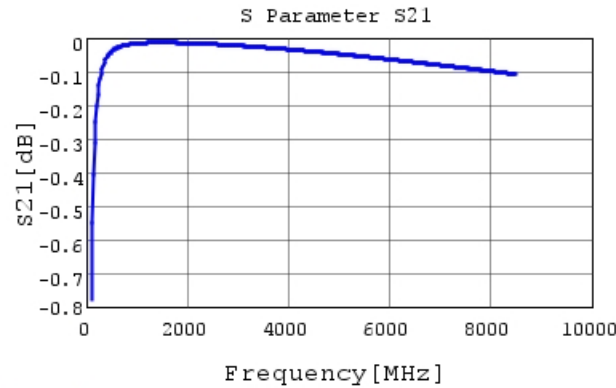
GRM0115C1E360GE01 S21 DCOV, 25degC
