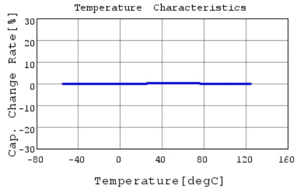
GRM0115C1E510JE01 C-Temp. capchange, DCOV, 1
