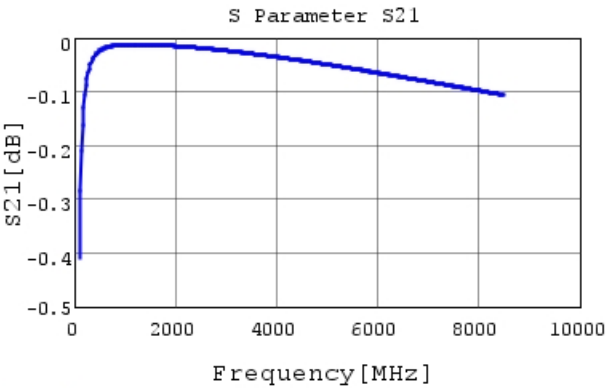
GRM0115C1E510JE01 S21 DCOV, 25degC
