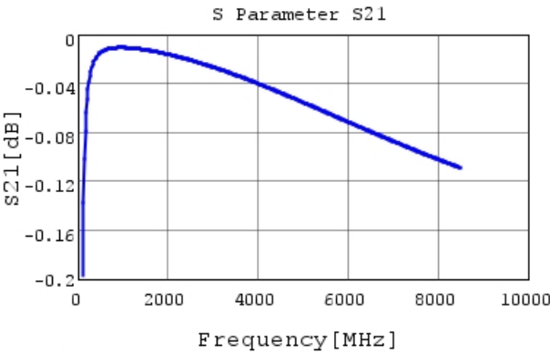
GRM0115C1E750GE01 S21 DCOV, 25degC
