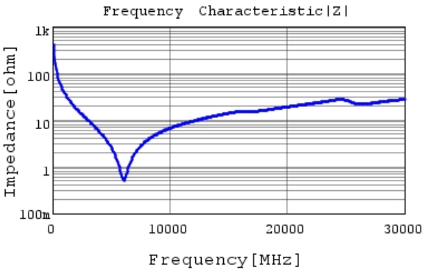
GRM0222C1H4R0WA03 |Z| DCOV,20degC
