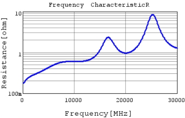
GRM0222C1H4R0WA03 R DCOV,20degC
