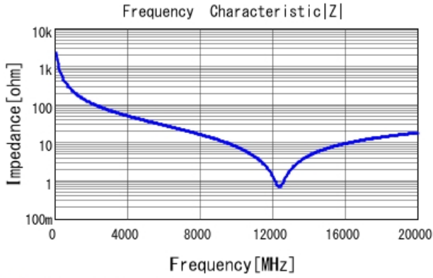
■ GRM0224C1HR70BA03 |Z| DCOV, 20degC
