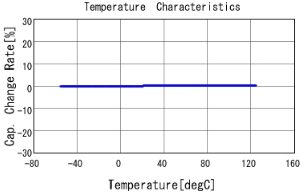
■ GRM0224C1HR70BA03 C-Temp. capchange, DCOV, AC1Vrms
