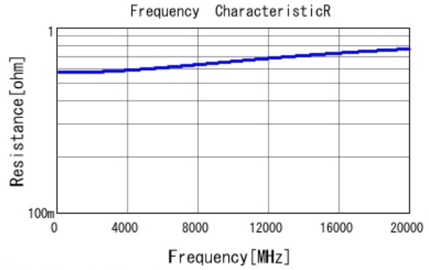
■ GRM0224C1HR70BA03 R DCOV, 20degC
