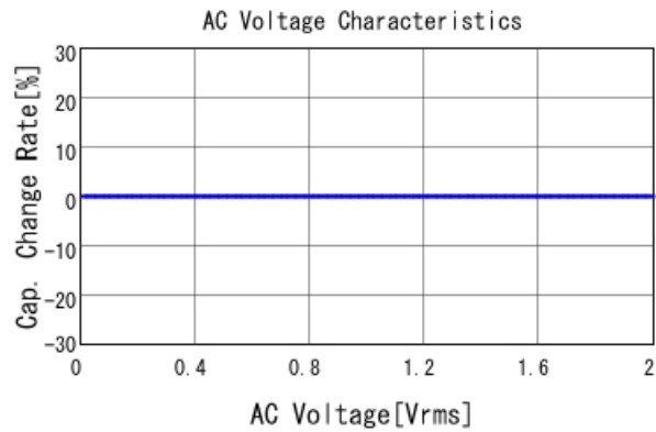
■ GRM0224C1HR70BA03 C-AC Voltage capchange, DCOV, 20.0d
