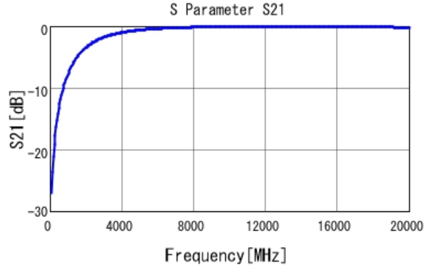
■ GRM0224C1HR70BA03 S21 DCOV, 20degC
