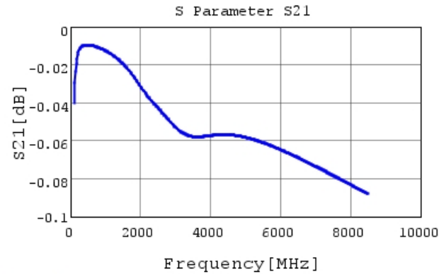
GRM0225C1E181JA02 S21 DCOV, 25degC
