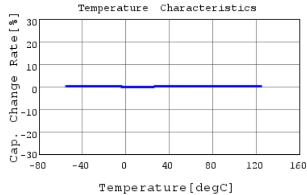
GRM0225C1E181JA02 C-Temp. capchange, DCOV, 1
