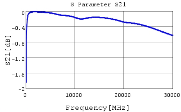
GRM0225C1E220GA02 S21 DCOV, 25degC
