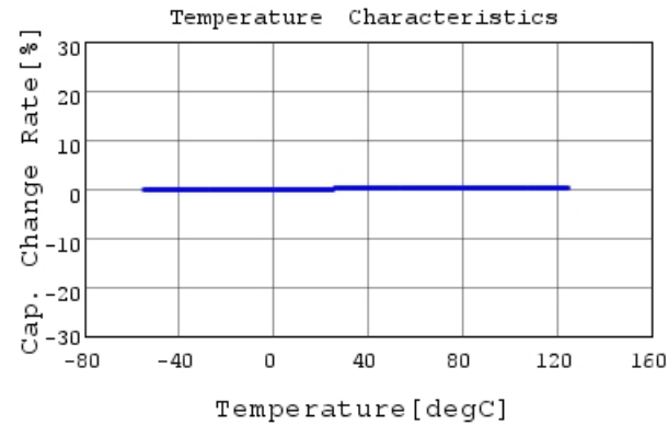
GRM0225C1E220GA02 C-Temp. capchange, DCOV, 1
