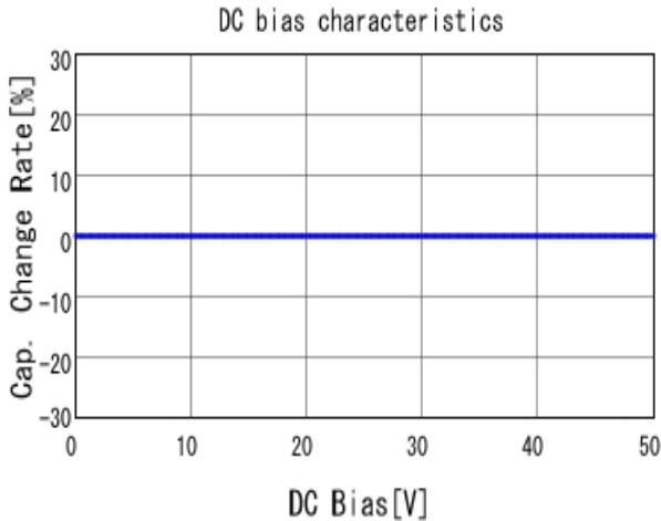
■ GRM0225C1H2R1WA03 C-DC bias capchange, 25.0degC, AC1V
