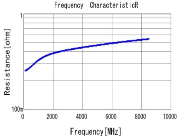
■ GRM0225C1H2R1WA03 R DCOV, 25degC
