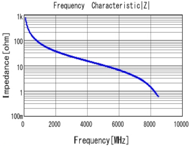
■ GRM0225C1H2R1WA03 |Z| DCOV, 25degC
