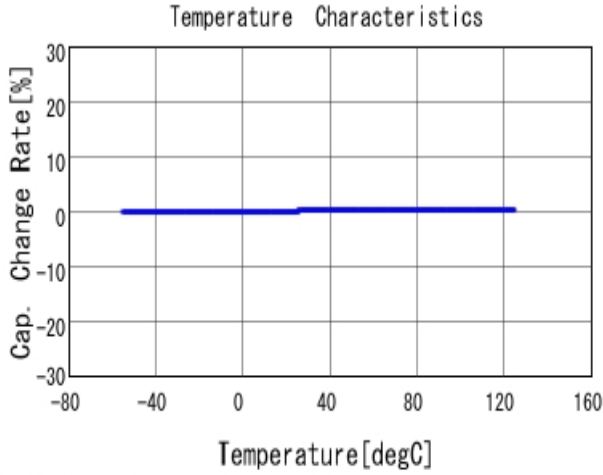
■ GRM0225C1H2R1WA03 C-Temp. capchange, DCOV, AC1Vrms
