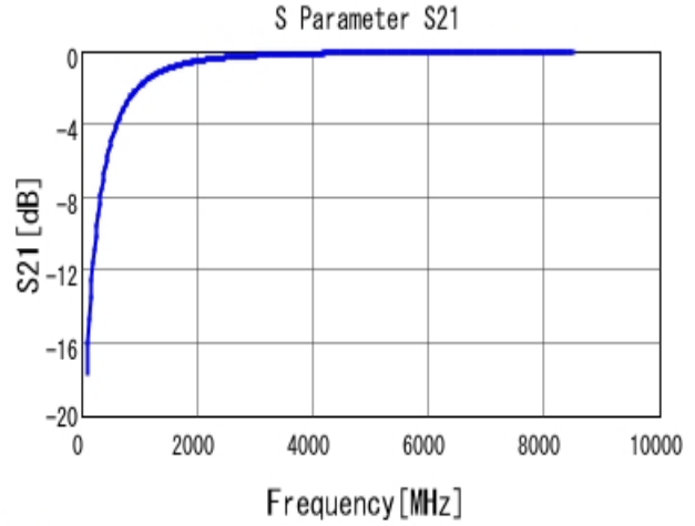
■ GRM0225C1H2R1WA03 S21 DCOV, 25degC
