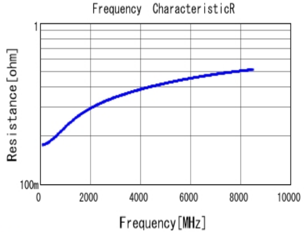
■ GRM0225C1H3R9BA03 R DCOV, 25degC
