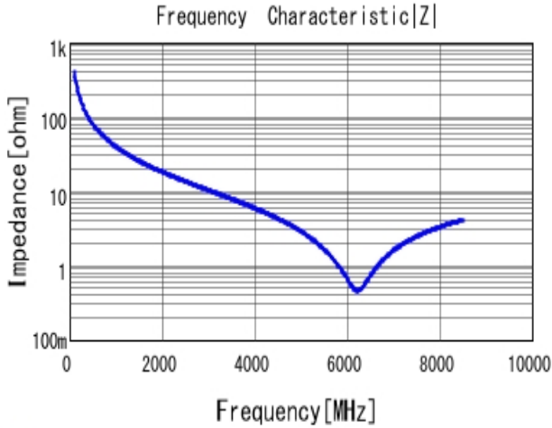
■ GRM0225C1H3R9BA03 |Z| DCOV, 25degC
