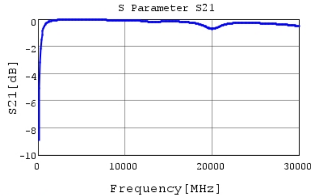
GRM0225C1H6R1DA03 S21 DCOV, 25degC
