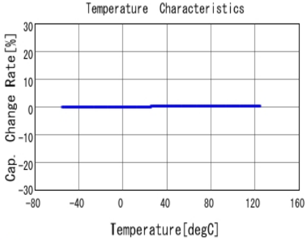
■ GRM0225C1H8R4CA03 C-Temp. capchange, DCOV, AC1Vrms
