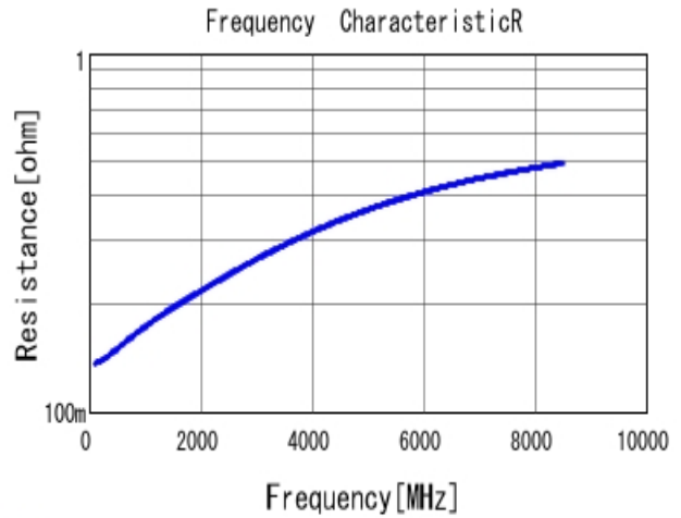
■ GRM0225C1H8R4CA03 R DCOV, 25degC
