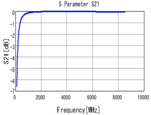
■ GRM0225C1H8R4CA03 S21 DCOV, 25degC
