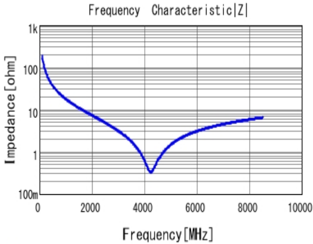
■ GRM0225C1H8R4CA03 |Z| DCOV, 25degC
