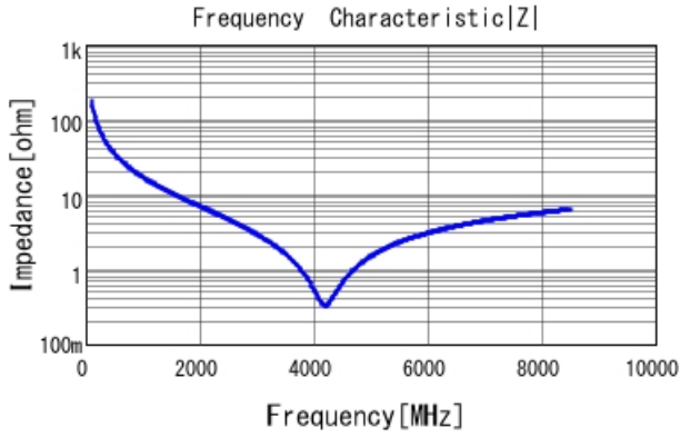
■ GRM0225C1H8R8DA03 |Z| DCOV, 25degC
