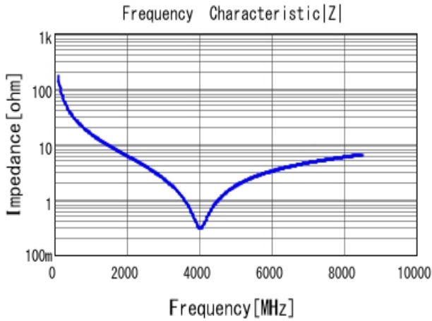
■ GRM0225C1H9R7BA03 |Z| DCOV, 25degC
