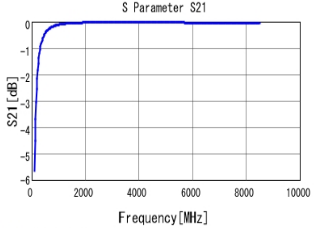
■ GRM0225C1H9R7BA03 S21 DCOV, 25degC
