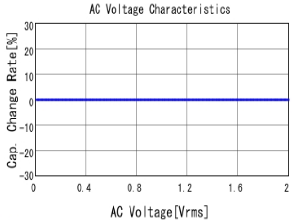
■ GRM0225C1H9R7BA03 C-AC Voltage capchange, DCOV, 25.0d
