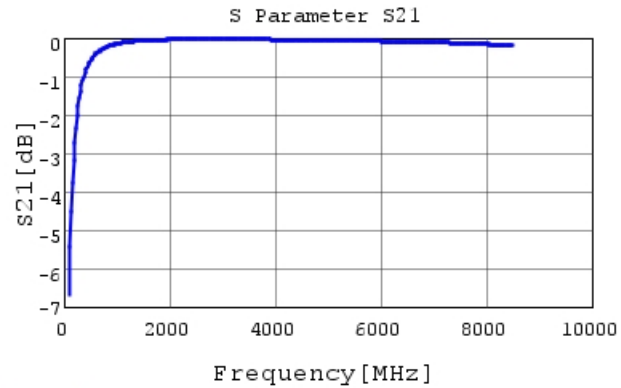
GRM0332C2A8R3WA01 S21 DCOV, 20degC
