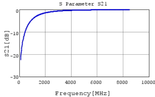
GRM0335C1H1R2CA01 S21 DCOV, 25degC
