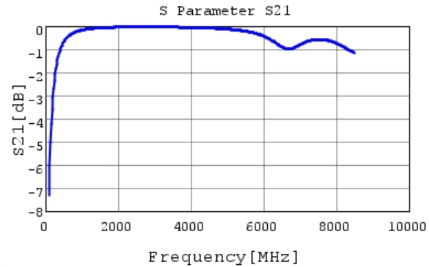
GRM1552C1H7R6CA01 S21 DCOV, 20degC
