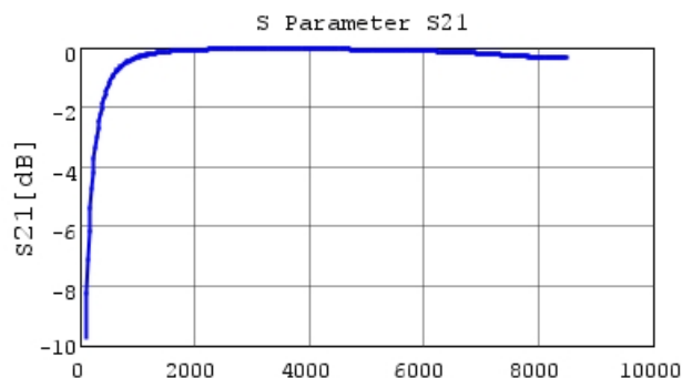
GRM1552C2A5R5DA01 S21 DCOV, 20degC
