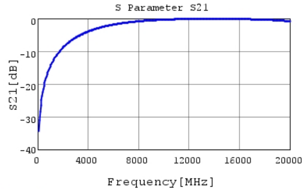
GRM1554C2AR30WA01 S21 DCOV, 20degC
