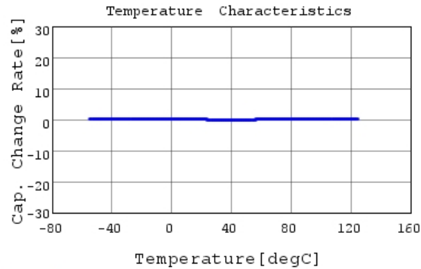
GRM1555C2A7R4DA01 C-Temp. capchange, DC0V, 1
