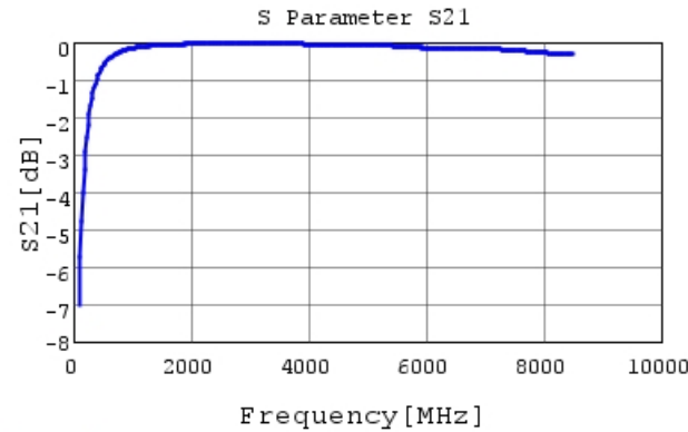
GRM1555C2A7R9CA01 S21 DC0V, 25degC
