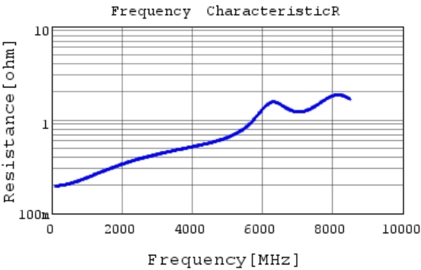
GRM1555C2A7R9CA01 R DCOV,25degC
