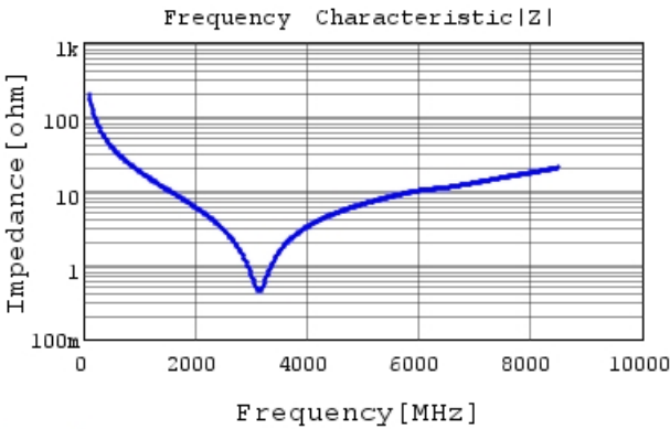
GRM1555C2A7R9CA01 |Z| DCOV,25degC
